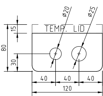
CONDUIT LOCATION TO SIDES (TYP.)
